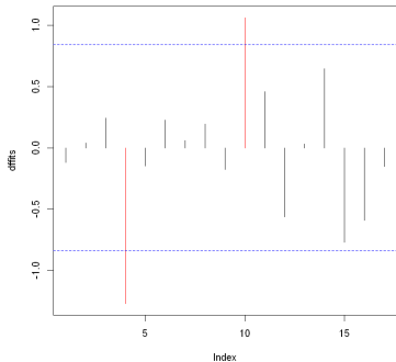
DFFITS
